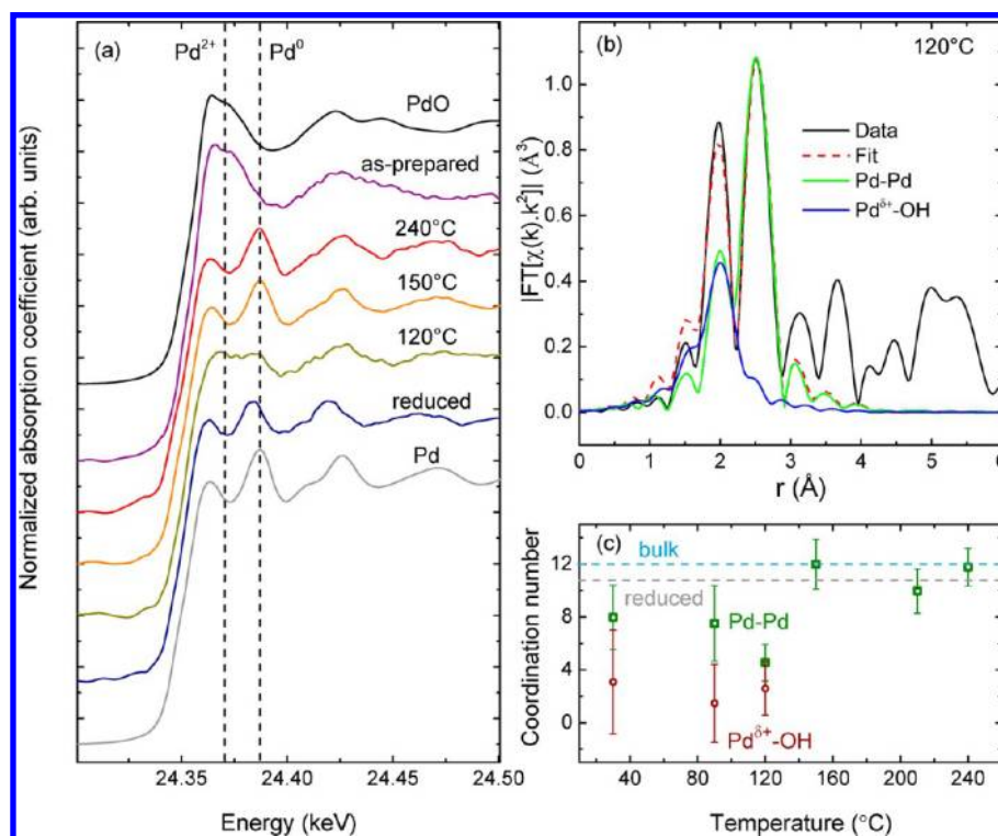
FIGURE 10. (a) Pd K-edge XANES spectra of micelle-synthesized Pd NPs on \text{ZrO}_2 taken after polymer removal in \text{O}_2 at 375^\circ\text{C} (as-prepared), after reduction in \text{H}_2 at 240^\circ\text{C} and subsequent cooling to RT (reduced), and at different temperatures during the NO reduction with \text{H}_2 . (b) Fourier transform Pd K-edge EXAFS spectrum ( r -space) recorded at 120^\circ\text{C} in \text{NO} + \text{H}_2 , along with the total fit and the Pd–Pd and \text{Pd}^{\delta+} –OH contribution. (c) Dependence of the 1st NN CN extracted from EXAFS data on the reaction temperature during the reduction of NO with \text{H}_2 . The dashed gray line indicates the Pd–Pd CN after NP reduction in \text{H}_2 and before reactant exposure.
