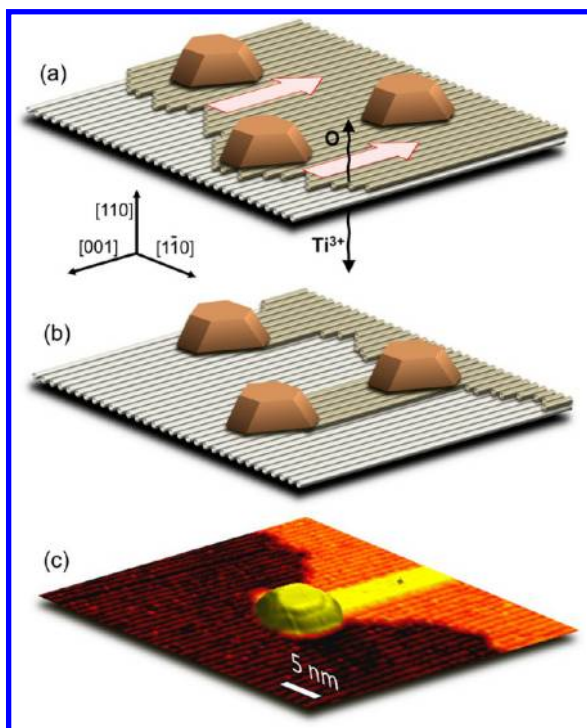
FIGURE 5. (a,b) Schematic representation of the formation of TiO 2 nanostripes stabilized by micellar Pt NPs. Oxygen desorption and inward diffusion of Ti 3+ (into the bulk of TiO 2 ) predominantly occurs at [1-10] step edges, while [001] steps remain stable. This results in the loss of unpinned TiO 2 rows starting from their free ends. Pt NPs can stabilize [1-10] steps and protect TiO 2 rows attached to them by those steps. The STM image in (c) displays a nanostripe–nanoparticle configuration.
