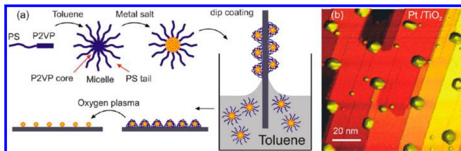
FIGURE 1. (a) Schematic description of the inverse micelle encapsulation NP synthesis. (b) STM image of Pt NPs on TiO 2 (110) acquired at RT after sample heating in UHV at 1000 °C.
