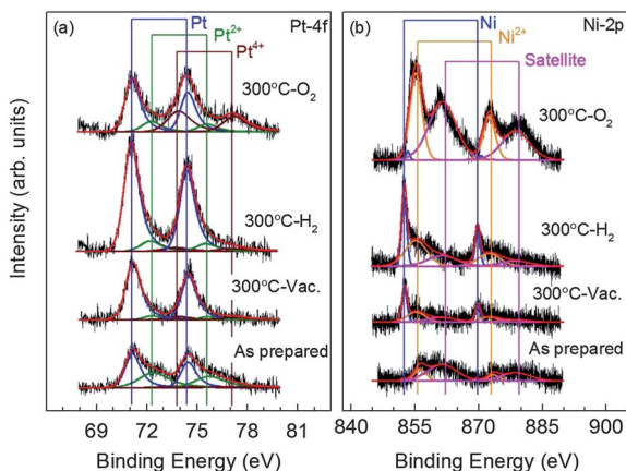
Fig. 5 XPS spectra from the (a) Pt-4f and (b) Ni-2p core level regions of PtNi NPs supported on HOPG acquired at RT before (as prepared) and after annealing in vacuum and in 1 bar of O 2 and H 2 at 300 °C for 20 min.
