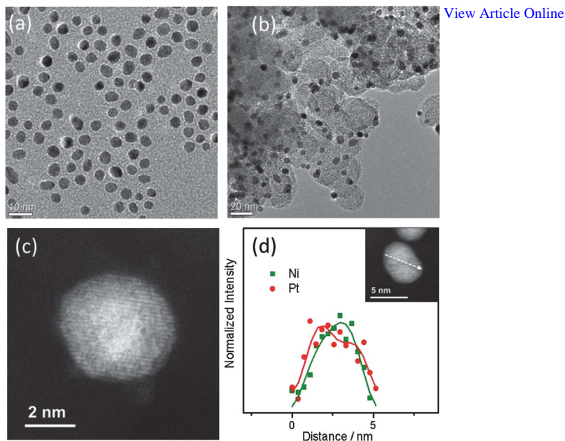
Fig. 3 TEM images of as-prepared spherical PtNi(s-PtNi) NPs: (a) unsupported s-PtNi, (b) carbon-supported s-PtNi, (c) HAADF-TEM image of an individual PtNi NP, (d) STEM EELS line scan (along the arrow in the inset) of a single PtNi NP showing the spatial distribution of Ni and Pt.
