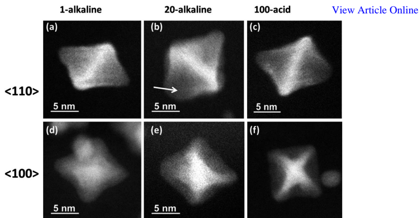
Fig. 8 (a) HAADF STEM images along the (a–c) \langle 110 \rangle and (d–f) \langle 100 \rangle zone axes of the three differently pretreated octahedral PtNi NPs (oct-PtNi/C): (a,d) “1-alkaline”, (b,e) “20-alkaline”, (c,f) “100-acid”.
