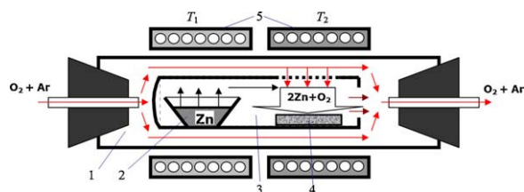
Fig. 1. Set-up of chemical vapor deposition for the growth of ZnO nanowires on a Si substrate: (1) flowing quartz reactor, (2) Zn source, (3) internal quartz retort, (4) substrates, (5) electric heaters.
