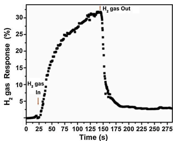
Fig. 11. Gas-response curve of the individual zinc oxide nanowire-based gas nanosensor under exposure to 100 ppm of \text{H}_2 gas at room temperature.
