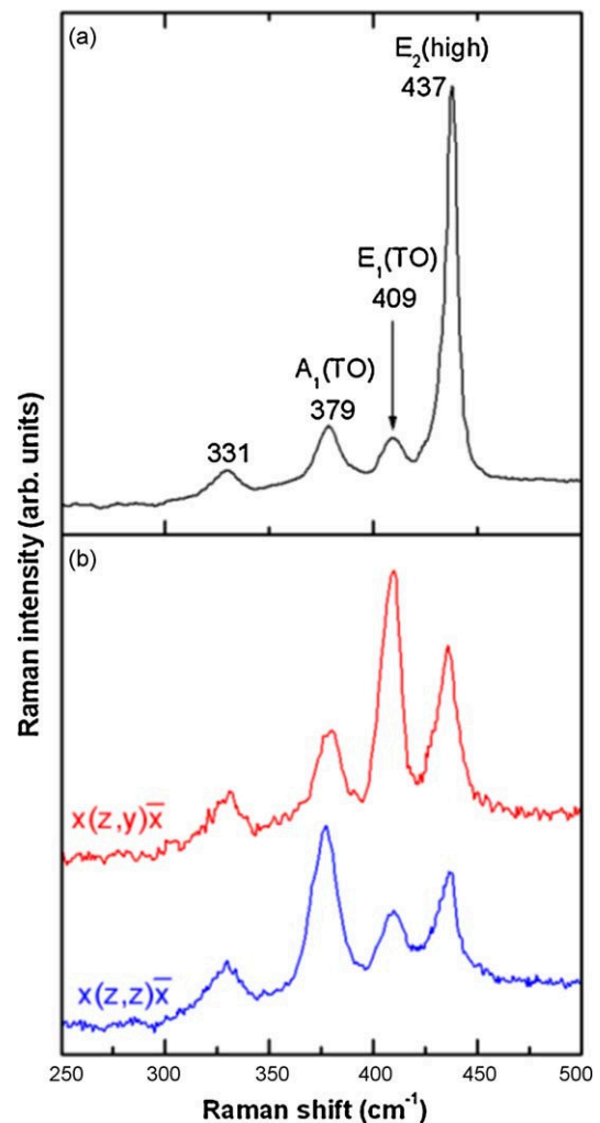
Fig. 9. Room temperature micro-Raman spectra of the ZnO nanowires: (a) non-polarized Raman spectrum measured in the quasi-backscattering geometry in the region of the TO phonons. (b) The polarized Raman spectra measured in-plane, i.e. from the edge of the sample (in the x -direction).
