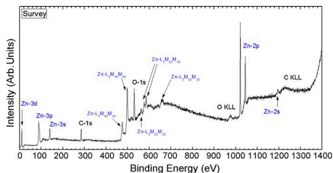
Fig. 5. Survey XPS spectrum corresponding to ZnO nanowires supported on SiO 2 /Si(0 0 1). Only Zn, O and adventitious C (from sample transport in air) are detected. The different photoelectron and Auger electron peaks (AES) peaks observed for the latter elements are labeled in the graph.
