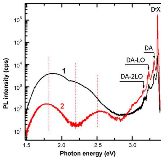
Fig. 7. Emission spectra of the ZnO nanowires with diameters of 50 nm (1) and 200 nm (2). T = 10 K.
