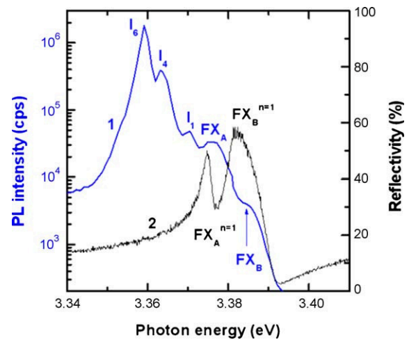
Fig. 8. The neutral donor- and free-exciton lines in the luminescence (1) and reflectivity (2) spectra of ZnO layers grown by CVD. T = 10 K.
