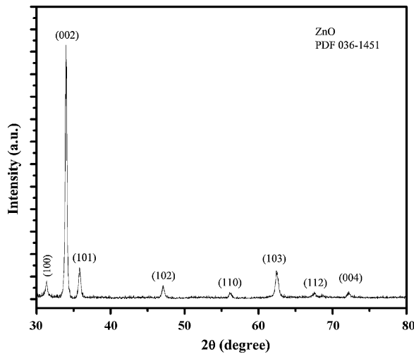
Fig. 2. XRD pattern of ZnO nanowires grown by CVD at 650 °C for 30 min. The indexing of the different XRD peaks was done using as reference a database from the Joint Committee on Powder Diffraction Standards, Powder Diffraction File No 36-1451.
