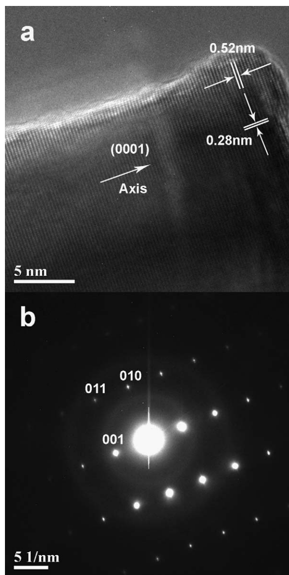
Fig. 4. (a) HRTEM image of ZnO nanowire grown by CVD method and (b) its corresponding selected area electron diffraction SAED pattern.
