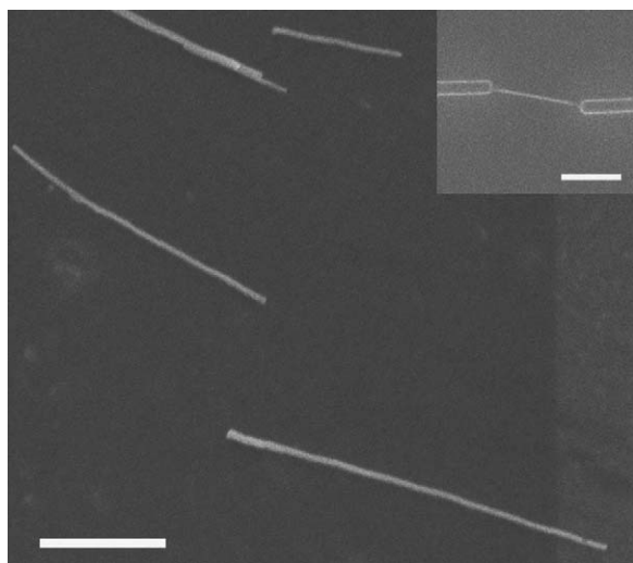
Fig. 10. Scanning electron micrograph of transferred ZnO nanowires. The insert shows device based on a single nanowire of 50 nm in diameter. Scale bars are 2\text{ }\mu\text{m} .
