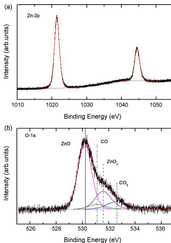
Fig. 6. XPS spectra (Al K \alpha = 1486.6 eV) corresponding to the (a) Zn-2p and (b) O-1s core level regions of ZnO nanowires supported on SiO 2 /Si(0 0 1).
