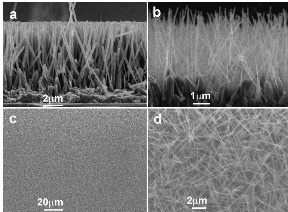
Fig. 3. SEM images of the cross-section of ZnO nanowire arrays with respect to the substrate position in the growth zone: (a) at the entrance of the growth zone (ratio O/Zn is larger), (b) at the exit of the growth zone (ratio O/Zn is smaller). Next are the SEM top-view images: (c) of the ZnO nanowires grown on ZnO/Si placed at the exit of zone (ratio O/Zn is smaller), (d) zoom in view image of the ZnO nanowires.
