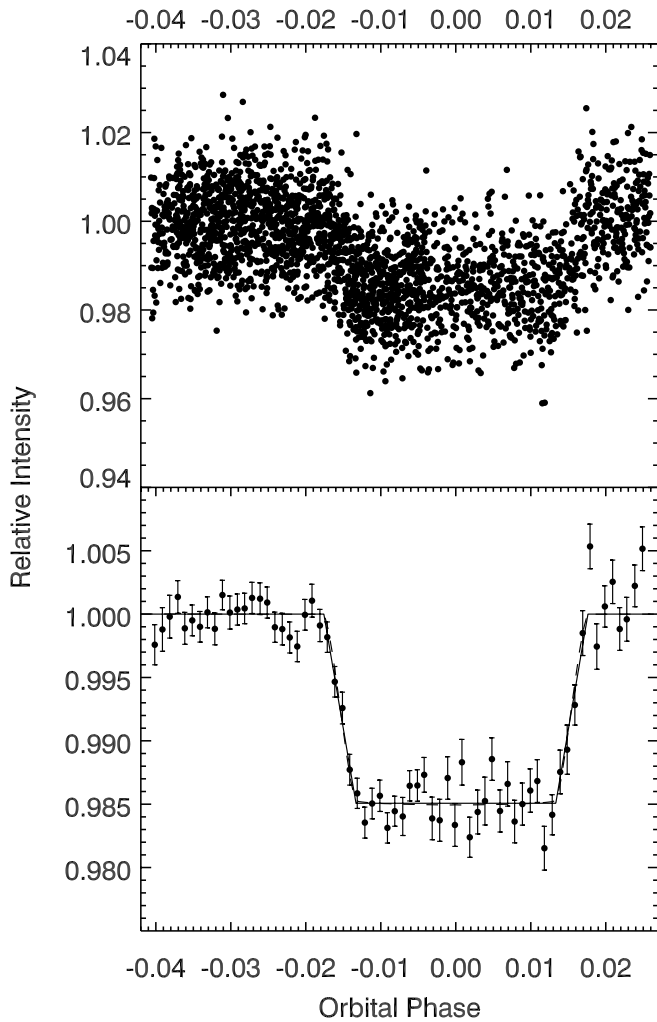
FIG. 1.— Top : All 2392 measurements vs. heliocentric phase. Bottom : Data averaged in phase (bin size = 0.001 in phase); also shown are the best-fit straight-line curve (solid line) and the exact theoretical light curve (faint dashed line), calculated using the best-fit physical parameters derived from the straight-line curve. Heliocentric phase was computed using the orbital period and ephemeris from Knutson et al. (2006).
