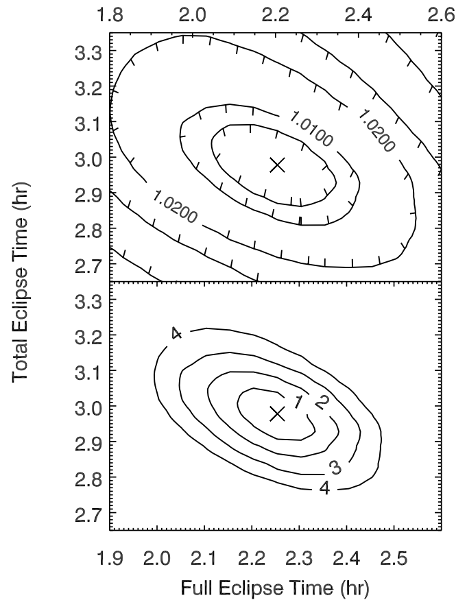
FIG. 2.— Top : Contour plot of the \chi^2_\nu fit from method 1, showing the total eclipse time vs. the full-eclipse time at zero phase offset (best-fit value). Bottom : Same result, but converted to confidence interval in standard deviations. In both panels, the minimum \chi^2_\nu (1.0051) is marked by a cross.
