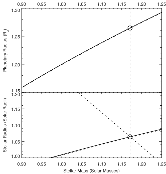
FIG. 3.—Stellar density derived from the best-fit parameters, transformed to stellar radius by assumption of a range of stellar masses. The transit data therefore yield an empirical mass-radius relation. Top : Planetary radius as a function of assumed stellar mass. Solid line represents result from MPFIT (method 2); dotted line represents the trial-and-error minimization technique (method 1). Bottom : Stellar radius as a function of assumed stellar mass. Methods 1 and 2 indicated as in top panel. Dashed line represents mass-radius relation from Cody & Sasselov (2002). Intersection of this relation with the empirical curve to the assumed stellar masses allows a determination of the stellar mass ( 1.171 M_{\odot} ), marked by the vertical dotted line. This reveals the best-fit stellar and planetary radii: R_{*} = 1.06 R_{\odot} and R_p = 1.26 R_{\oplus} .
