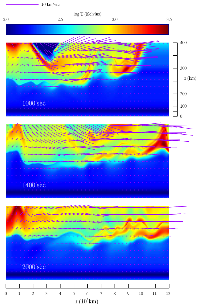
Figure 8.11. See Plate 6. Atmospheric plume landing response model. Color is temperature and anchored streamers show flow. The McGregor's ring shock is leaving the right edge of the grid, while the vanguard makes its final reentry near the origin in the 1000 s panel. z=0 is 1 bar pressure. Reprinted from Deming and Harrington (2001).
