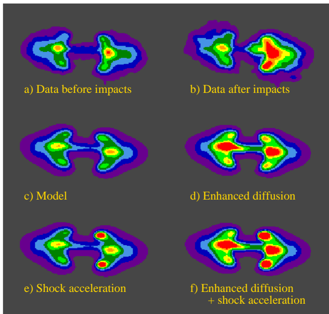
Figure 8.14. Real and model synchrotron emission images of Jupiter. a: 20-cm pre-impact VLA data. b: 20-cm VLA data taken after impact L. c: Synthetic 20-cm image from the Brecht et al. (2001) model using the ambient relativistic electron distribution. d: Synthetic 20-cm image with the diffusion coefficient enhanced by 3 \times 10^6 compared to panel c. e: Synthetic image after the interaction of a shock with the particle distribution in panel c. f: Synthetic image using both the shock model and enhanced diffusion. Reprinted from Brecht et al. (2001), copyright © 2001, with permission from Elsevier.
