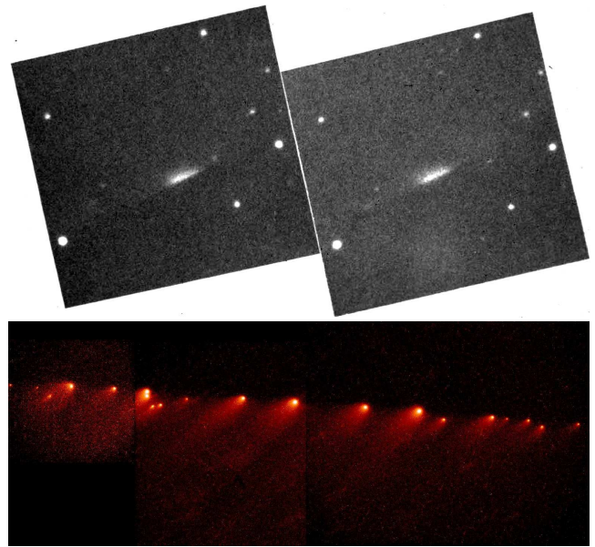
Figure 8.2. See Plate 6. Top: SL9 discovery image. Courtesy C. Shoemaker and D. Levy. Bottom: HST image of SL9 before impact. Courtesy H. Weaver and T. E. Smith (STScI) and NASA.
