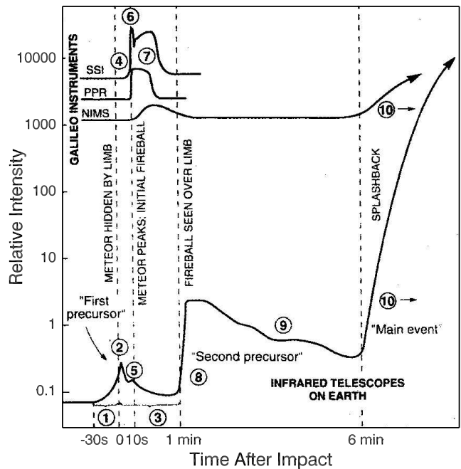
Figure 8.4. Schematic of the early light curves. 1–3: coma meteor shower (also called leader emission), 4 & 6: bolide entry, 5: possible reflection of bolide emission on trailing coma dust, 7: fireball, 8: plume becoming visible over limb, 9: cooling plume, 10: plume reentry. Adapted from Chapman (1996).
