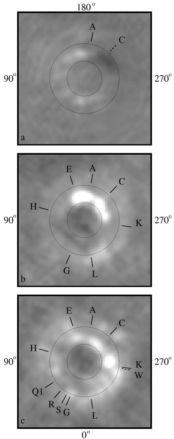
Figure 8.15. A 3D tomographic reconstruction of data taken with the Australian Telescope Compact Array on (top to bottom) July 17, 20, and 22, 1994. These are cuts through the dipolar magnetic equator of Jupiter (viewed from the north pole) showing the changes that occurred between the date shown and 5 days earlier. Border labels give magnetic longitudes and letters indicate the impact longitudes. The two circles are at 1 and 2 Jupiter radii. The brightness scale is the same for the three images. These images show that Jupiter’s synchrotron radiation brightened considerably in localized regions after specific impacts. Reprinted from Sault et al. (1997a), copyright © 1997, with permission from Elsevier.
