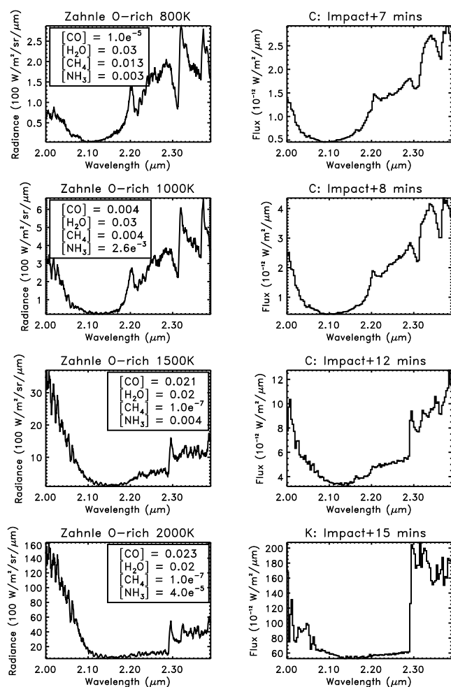
Figure 8.13. Comparison of observed spectra (right) with synthetic spectra (left). The synthetic spectra derive (Meadows et al. 2004) from O-rich splash model compositions as a function of peak shock temperature (Zahnle 1996, Figure 15). The early stages of the ejecta reentry are modeled with emission from CO, CH 4 , H 2 O and NH 3 at 800–1000 K (first two sets of panels). Although there is a good morphological match overall, in the range 2.32–2.36 μm there is an unexplained discrepancy. In the third set of panels (1500 K shock), the data and model both show the NH 3 plateau between 2.2 and 2.29 μm, and the sharp rise at 2.29 μm due primarily to hot CO emission. Water emission can also be seen at 2.29–2.40 μm, with a distinct feature at 2.385 μm, and at 2.0–2.09 μm. However, at the higher temperatures (1500–2000 K), the relative intensities of the two modeled H 2 O emission regions do not match those observed. Decreasing the relative abundance of H 2 O from the model values does not resolve this discrepancy. In the final set of panels (2000 K), note the sharp rise of the CO (2.295 μm) compared to the NH 3 plateau. The match of gross features and the evolution of features with time/temperature indicate that much of the variability observed is driven by chemical changes in the reentering ejecta as a function of increasing temperature. Reprinted from Meadows et al. (2004).
