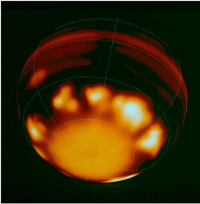
Figure 8.3. See Plate 6. Remapped composite of impact site images taken at 2.3\ \mu\text{m} at the Palomar 5-meter telescope. In this strong \text{CH}_4 band, stratospheric aerosols deposited by the impacts stand out against the dark troposphere. Note also the high-altitude hazes above the south pole and the Great Red Spot.
